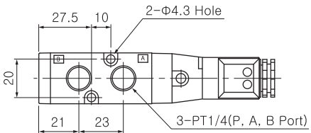
2position / 5port single(Lamp type)
