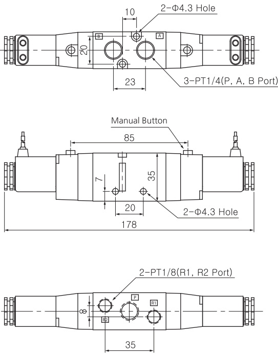
2position / 5port double(Grommet type)
